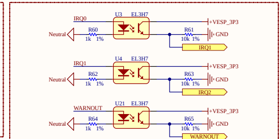
STATUS & INTERRUPTS - ISOLATED
