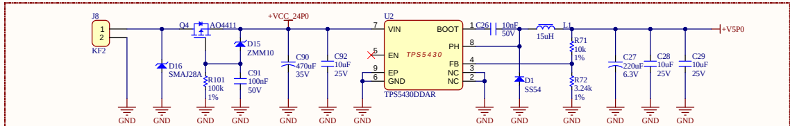
POWER SWITCHING
