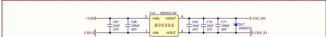
IO POWER - ISOLATED
